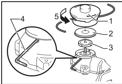
► 1. Nylon cutting head 2. Metal guard 3. Receive washer 4. Hex wrench 5. Tighten
